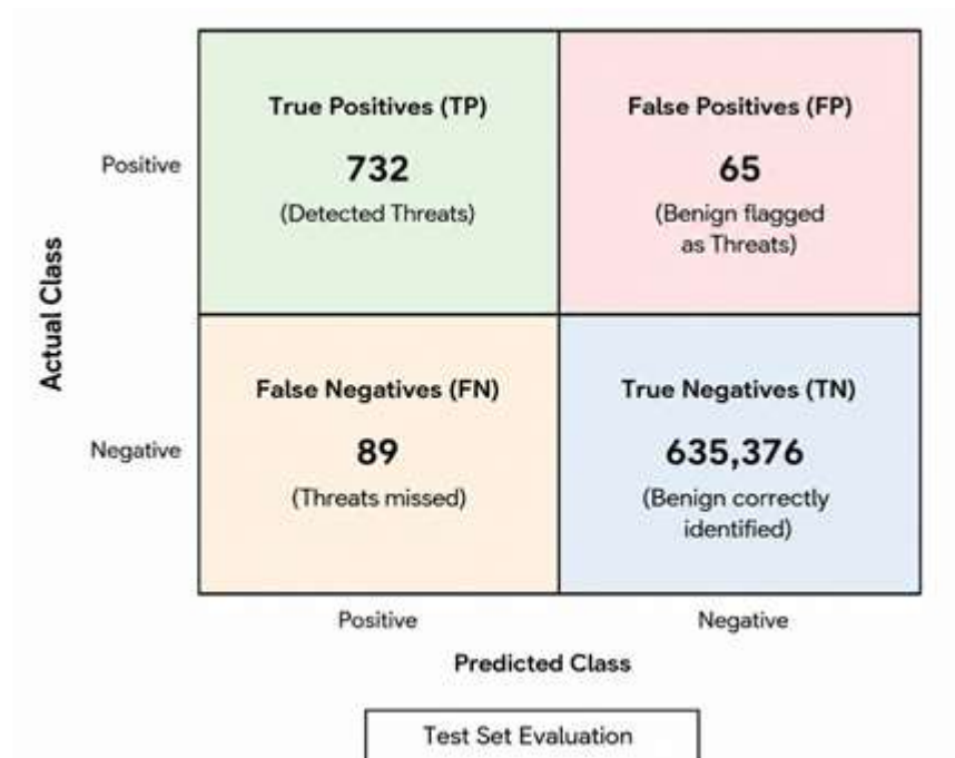
Figure 2: Confusion Matrix of Hybrid Detection Model
