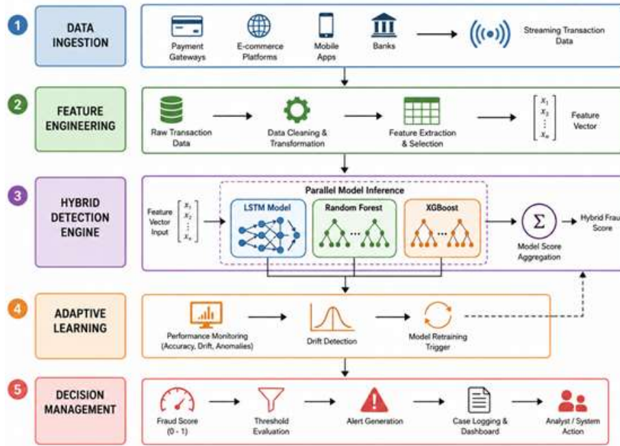
Figure 1: Proposed Framework Architecture Diagram
